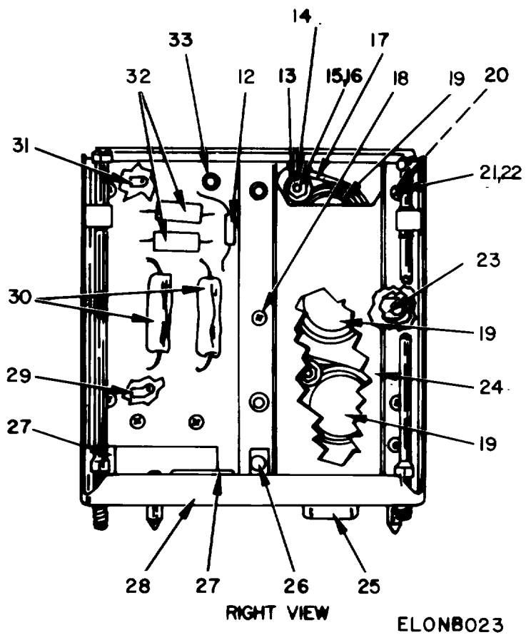
Figure 23. Amplifier.
